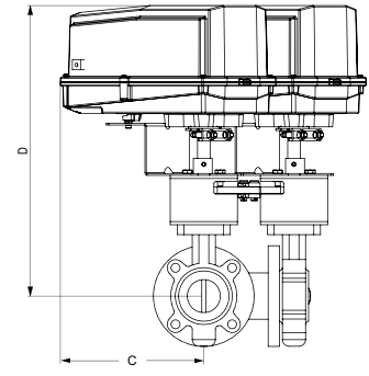
Valve Nominal Size Dimensions (Inches [mm])
